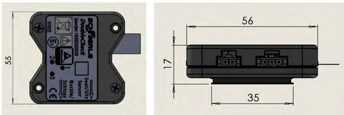
Dimensions Transmitter
